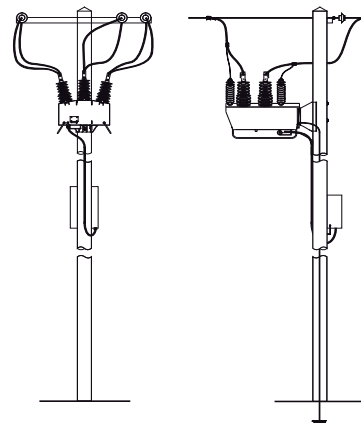
THREE PHASE POLE MOUNTING ARRANGEMENT
